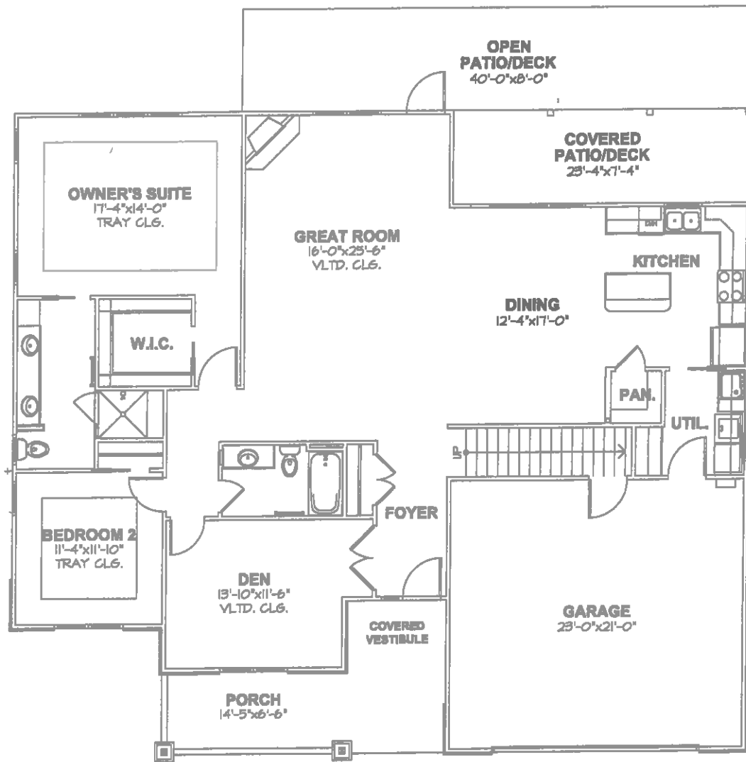
MAIN FLOOR PLAN SCALE: 1/8" = 1'-0"
